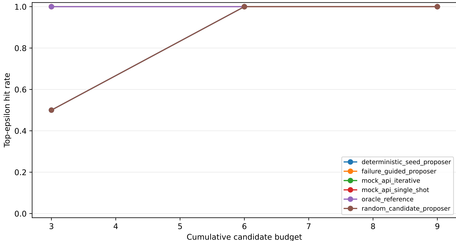
Iterative agent budget efficiency
