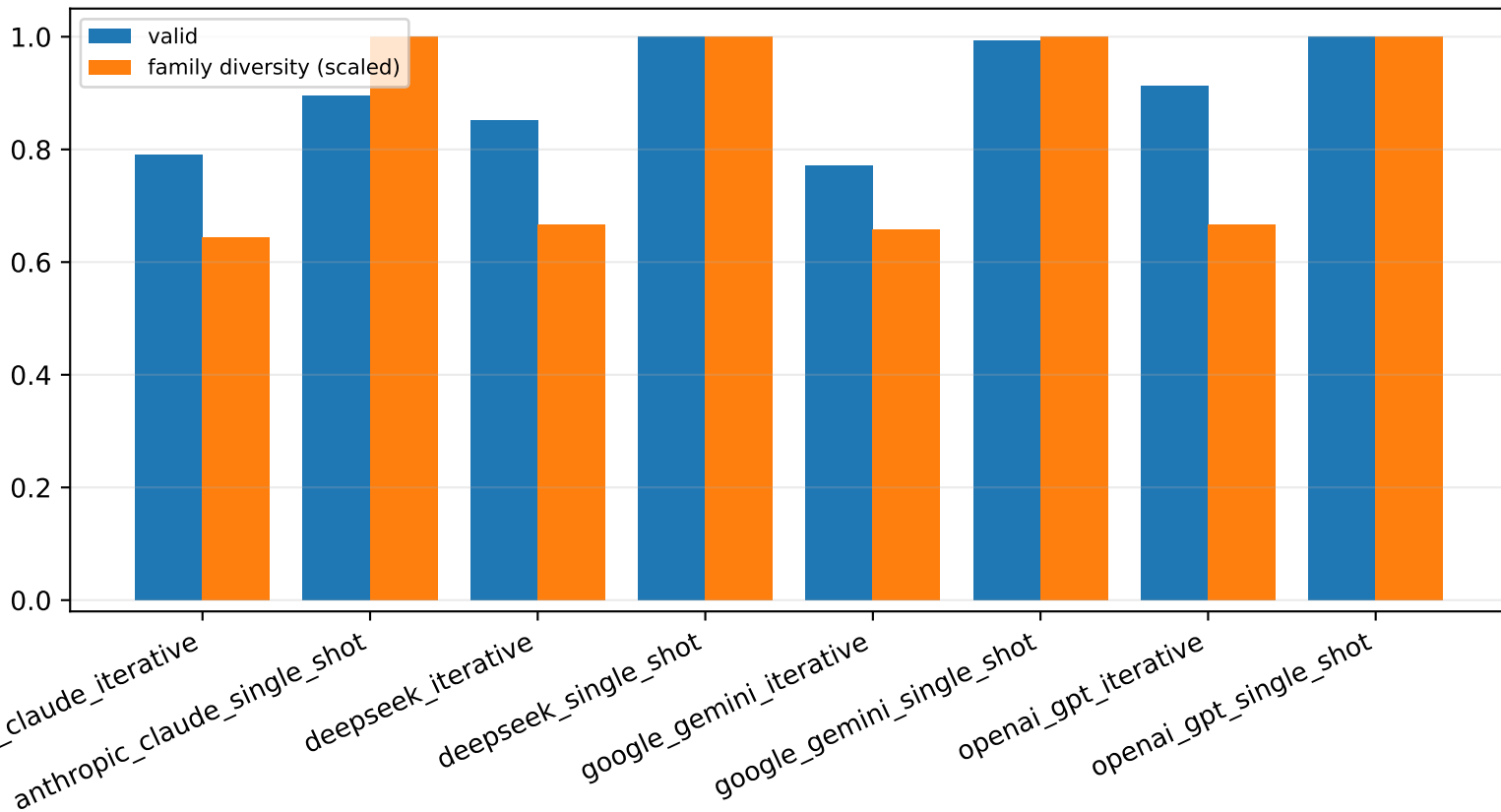
Provider structured proposal validity and diversity
