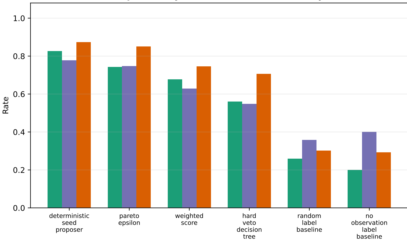
Observation Delay Top-epsilon Expanded synthetic structured recovery
