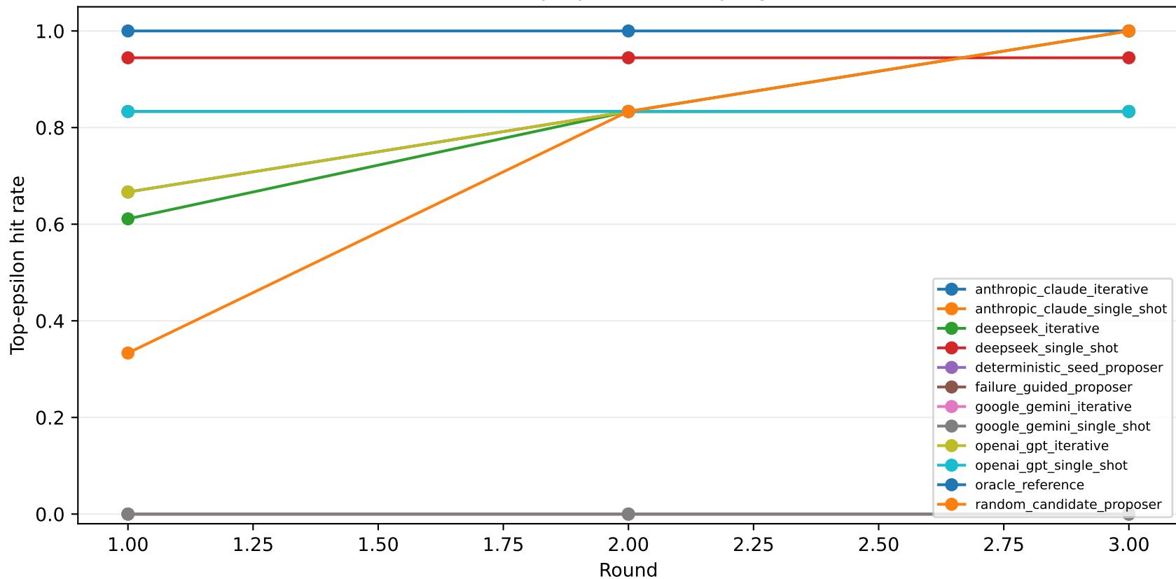
Provider proposer round progress
