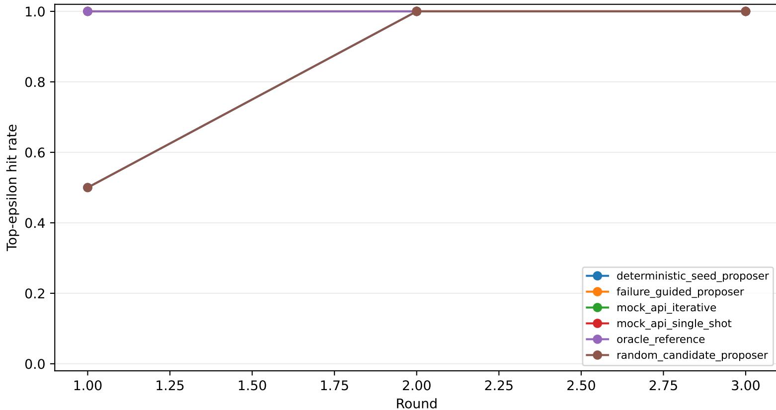
Iterative agent loop progress by round
