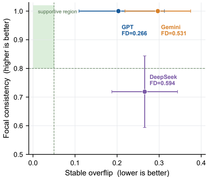
b Correct focal flips do not imply stable decisions
