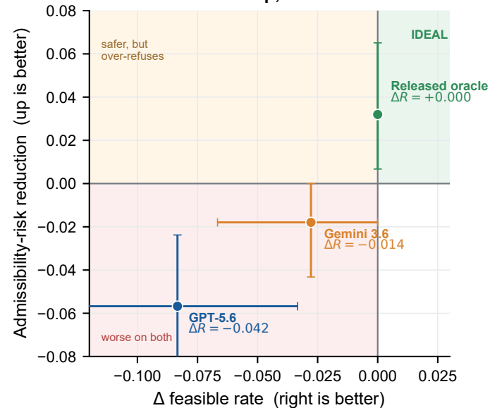
a Released fields help; text inference does not
