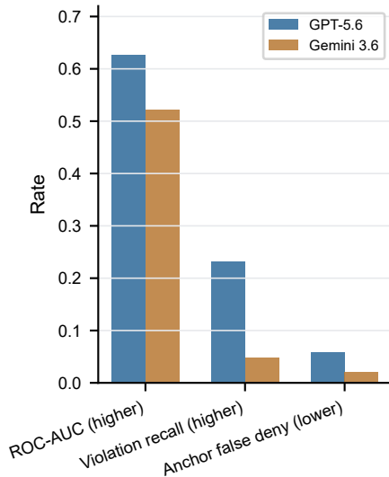
b Natural text inference is weak
