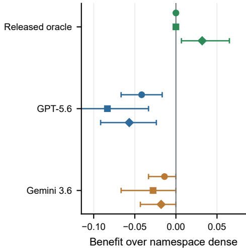
a Oracle headroom is unrealized
