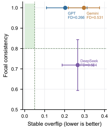
c Rule-following is not selectivity
