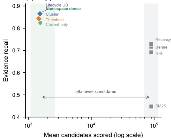
(c) Unresolved labels keep the upper bound high
