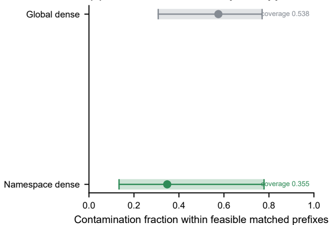
(c) Unresolved labels keep the upper bound high
