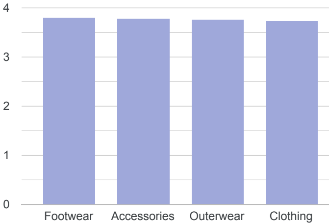
Review Rating
