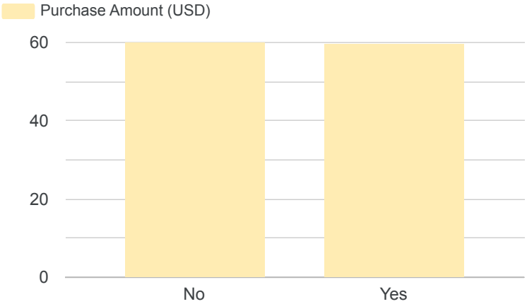
Subscription Impact
