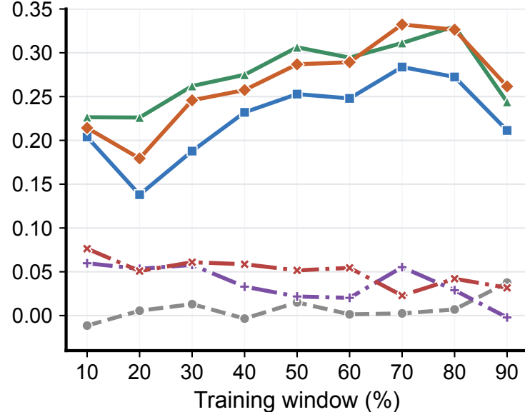
MCC
