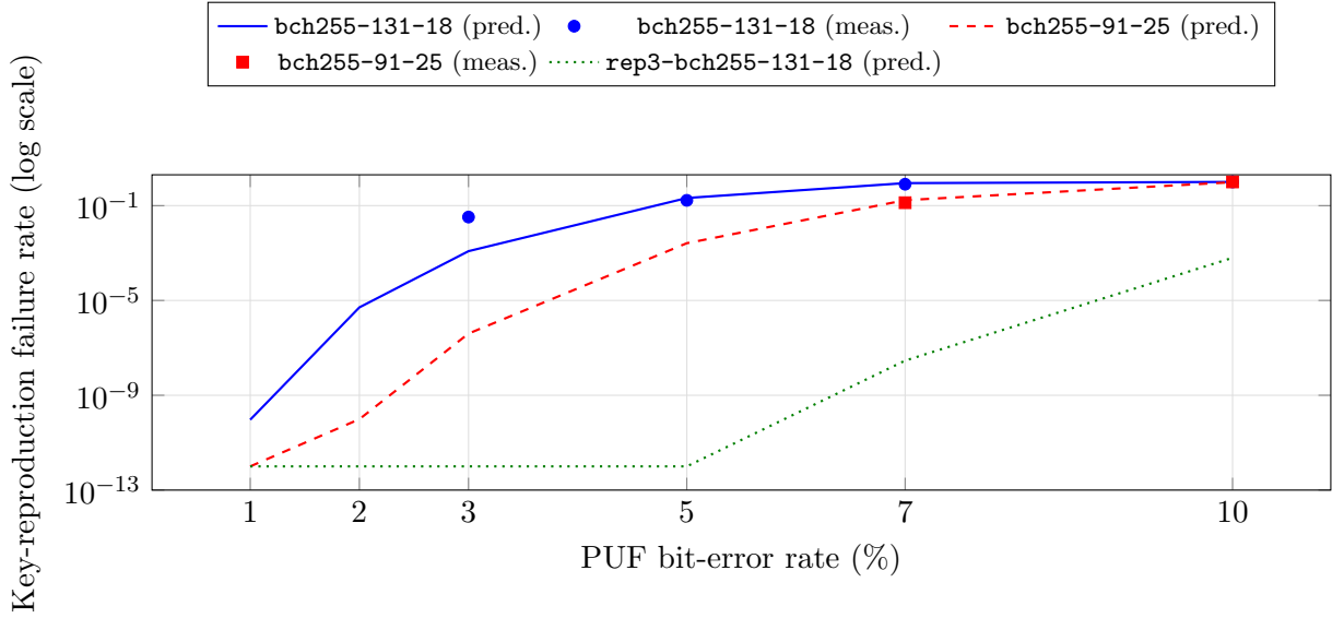
Figure 5: Measured key-reproduction failure rate against the analytic binomial prediction 1 - (1 - \Pr[\text{Bin}(255, p) > t])^L (data: Table 11). Measured points at 0.000 are omitted, since a rate of exactly zero has no representation on a log axis; every such point occurs where the predicted curve is also far below the 1/30 detection floor of a 30-device sample, so the omission does not hide disagreement. No measured marker is shown for rep3-bch255-131-18 because it measured zero failures at every tested bit-error rate, consistent with its curve remaining several orders of magnitude below the other two throughout the swept range.
