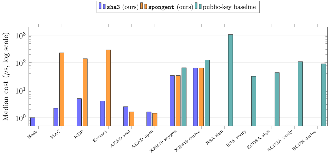
Figure 4: Median per-call cost, this work’s own primitives against public-key baselines, one logarithmic axis (data: Table 9). No bar is drawn for spongent Hash, matching the “—” in the table (HMAC’s nested structure is not defined over SPONGENT’s two-byte rate, so the sponge profile authenticates via a keyed sponge rather than a standalone hash call). The two X25519 categories each carry three bars because the operation is measured under both conditions described in the table’s footnote.
