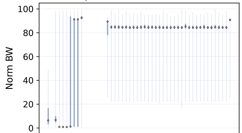
nic-only AllGather 32r/32n 12.87 MiB
