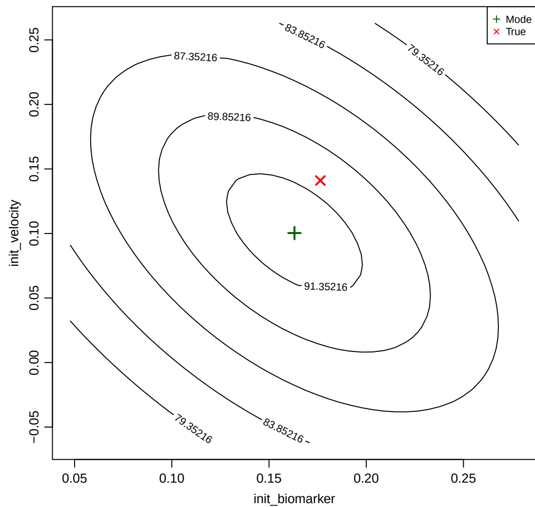
Subject 153: init_bio vs init_vel
