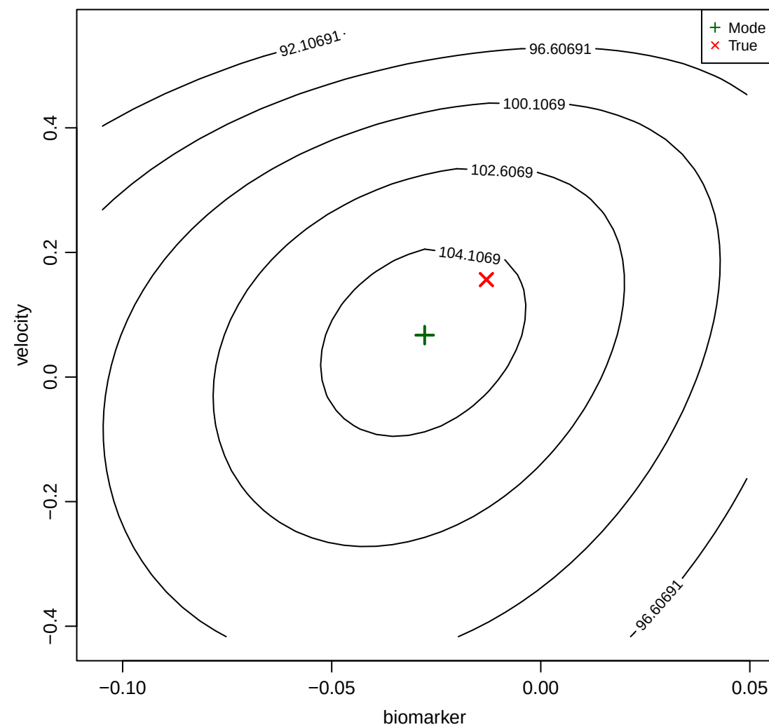
Subject 65: biomarker vs velocity
