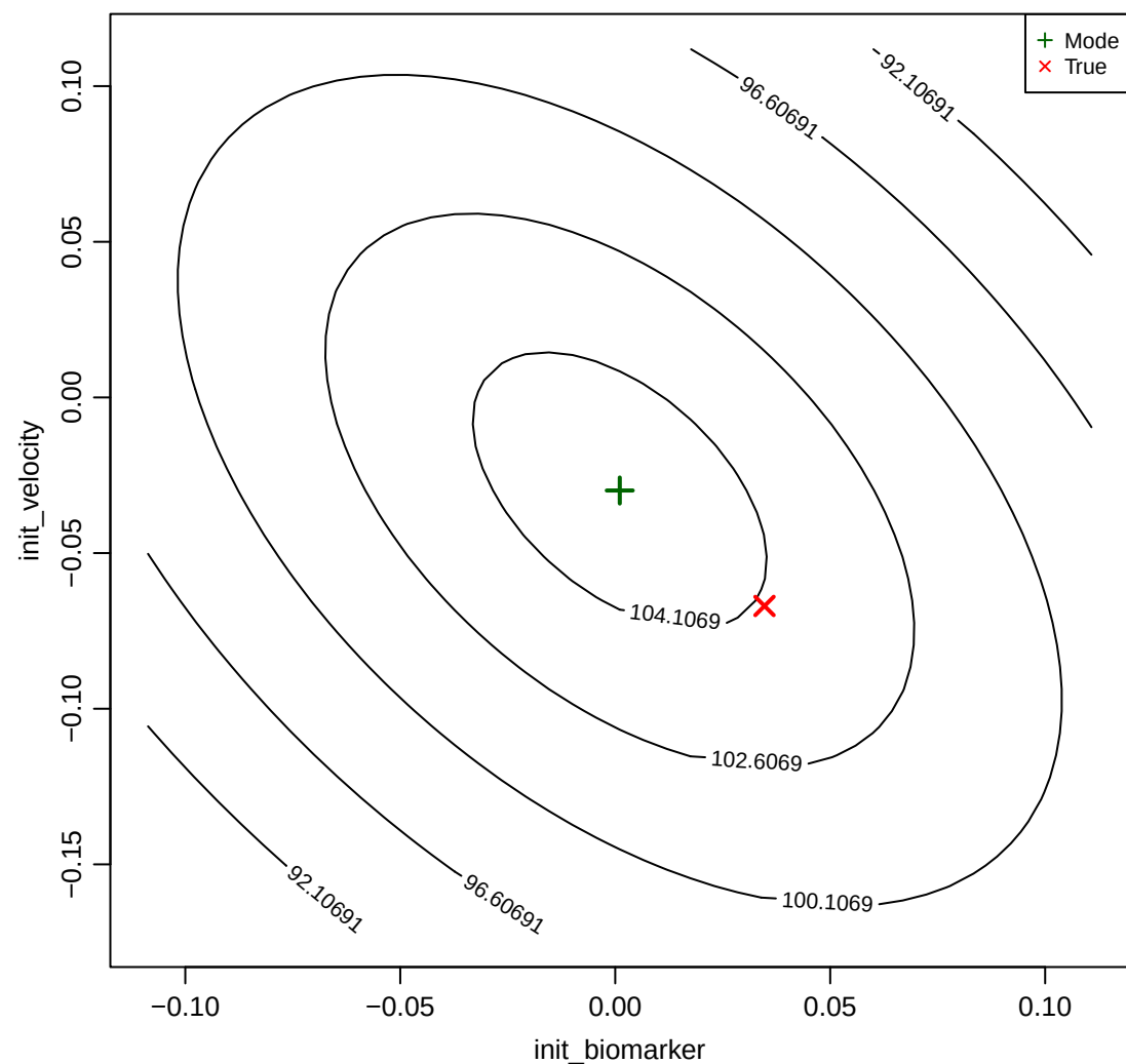
Subject 65: init_bio vs init_vel
