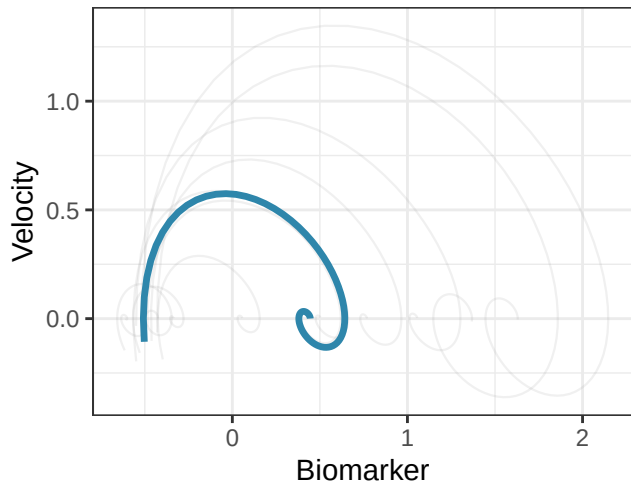
Phase Space
