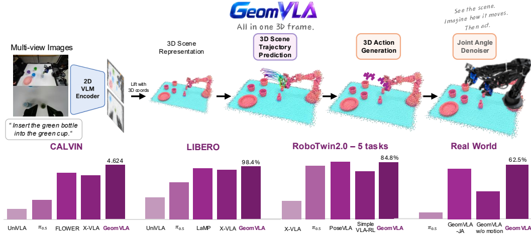
Figure 1: GeomVLA enables motion-guided 3D visual-language-action learning by bridging perception, latent future motion, and robot control in a shared 3D space. It lifts pretrained 2D VLM features into a geometrically grounded 3D representation, predicts latent 3D scene trajectories as an intermediate reasoning signal, and conditions a 3D action denoiser on the resulting scene-motion representation to generate robot actions. This design improves performance in both simulation and the real world. It also supports joint-angle action denoising by conditioning on scene-motion and end-effector pose-action features.
