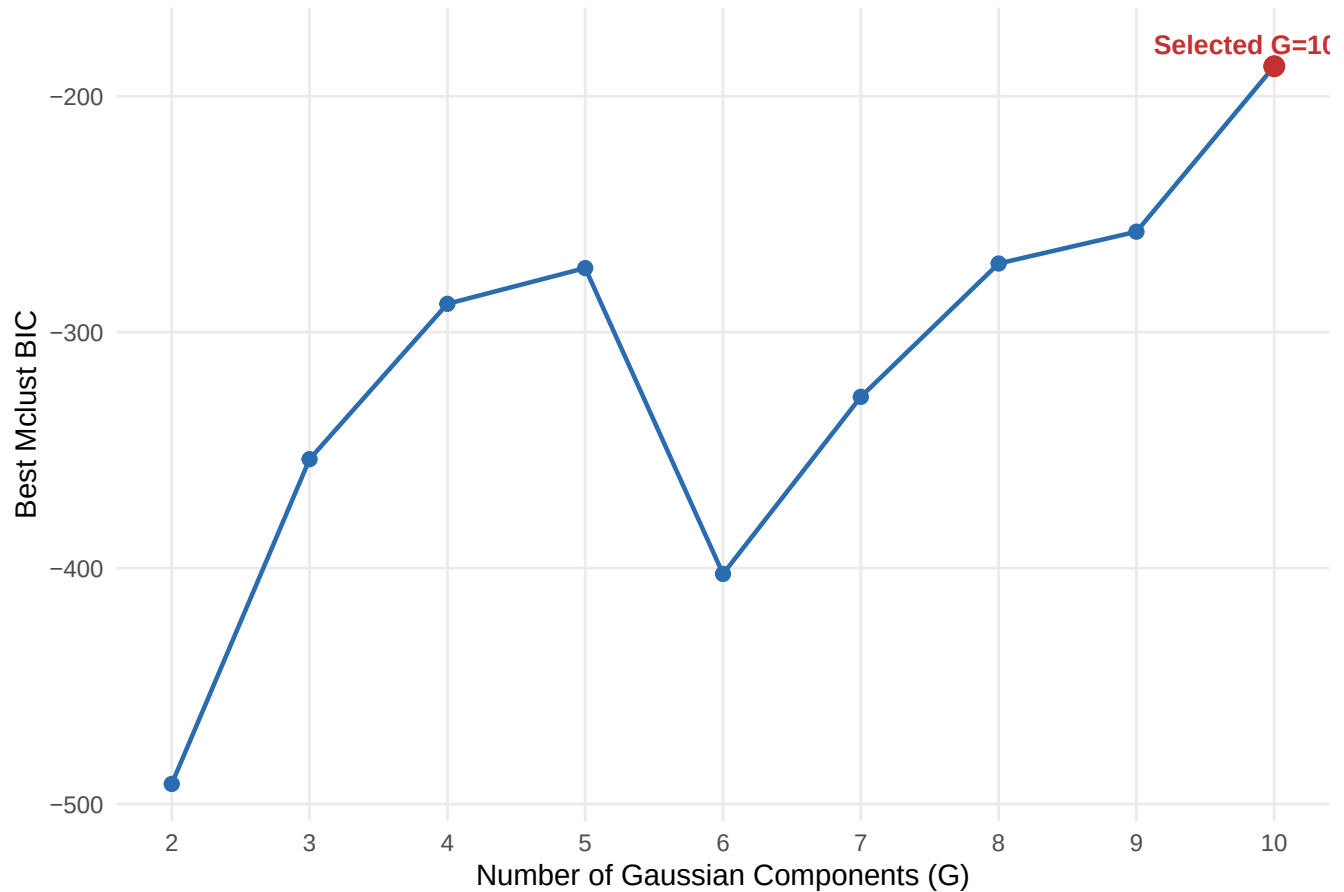
Gaussian Mixture Elbow Plot (combined, unweighted, target=Family, sideC
