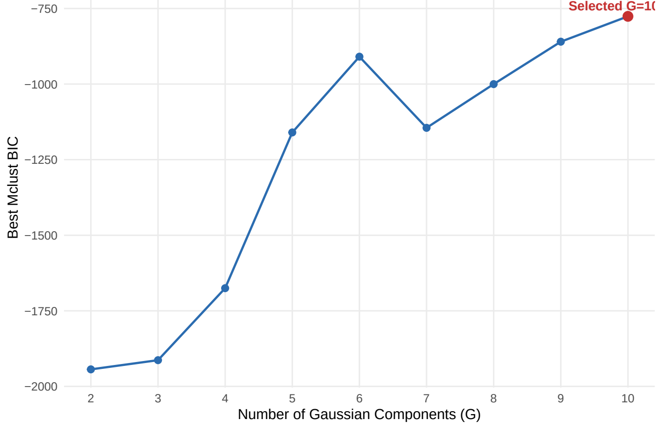
Gaussian Mixture Elbow Plot (combined, unweighted, target=Species, side
