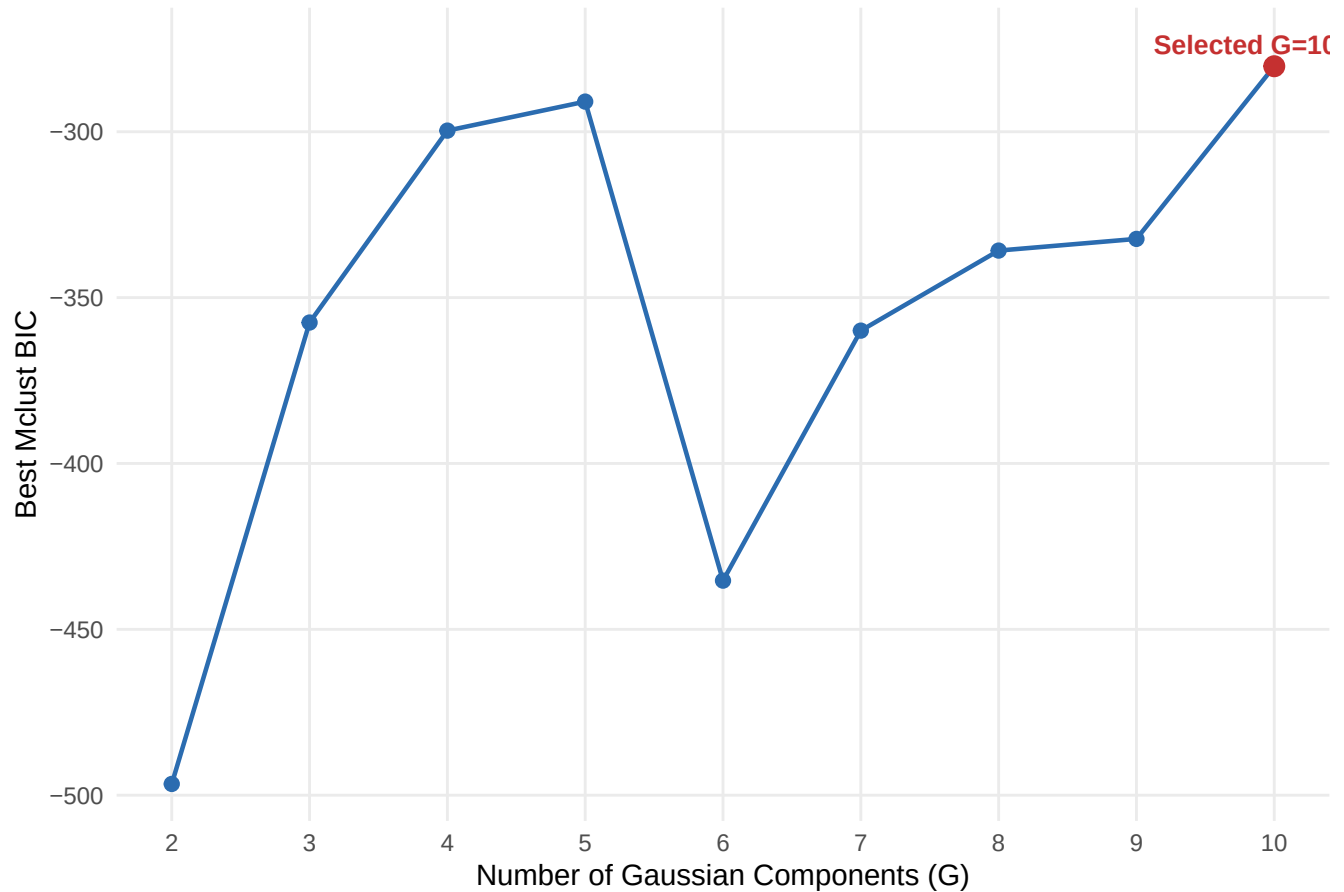
Gaussian Mixture Elbow Plot (combined, weighted, target=Family, sideCov
