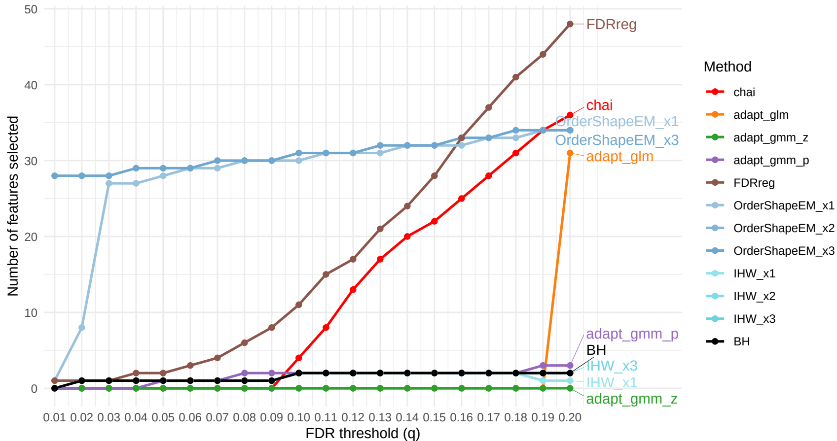
Feature Selection vs FDR (combined, unweighted, target=Family, sideCov=Class)
