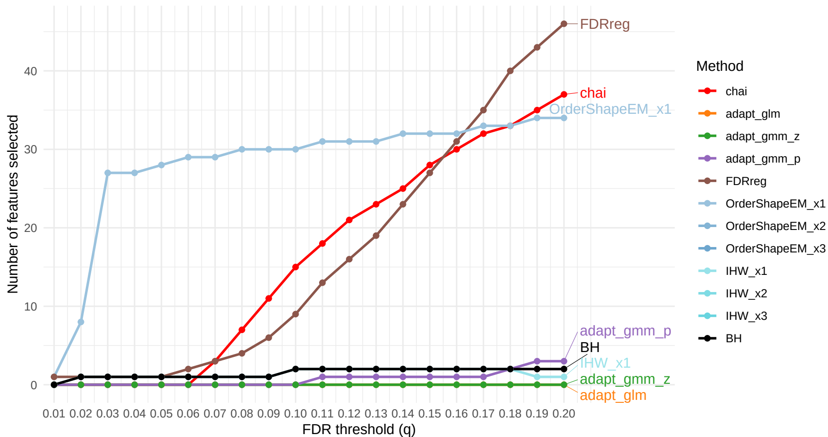
Feature Selection vs FDR (combined, unweighted, target=Family, sideCov=Family)
