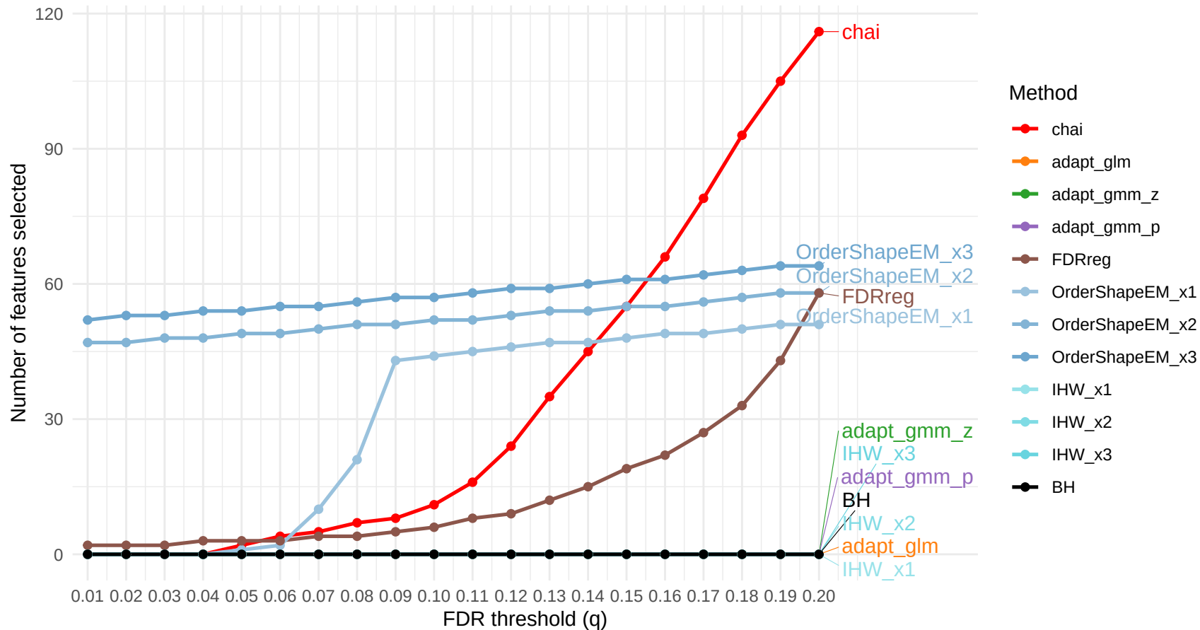
Feature Selection vs FDR (combined, unweighted, target=Genus, sideCov=Phylum)
