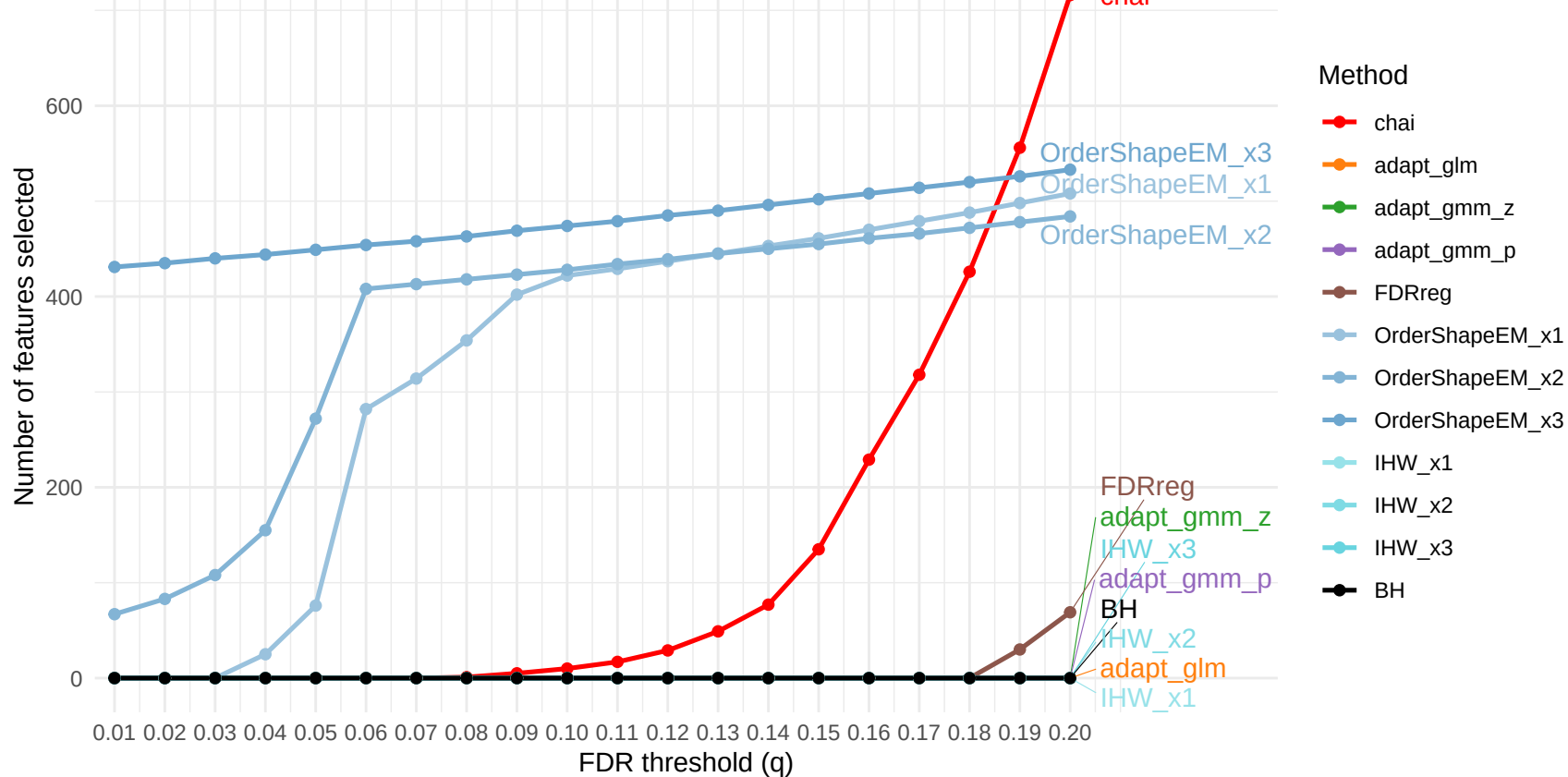
Feature Selection vs FDR (combined, unweighted, target=OTU, sideCov=Class)
