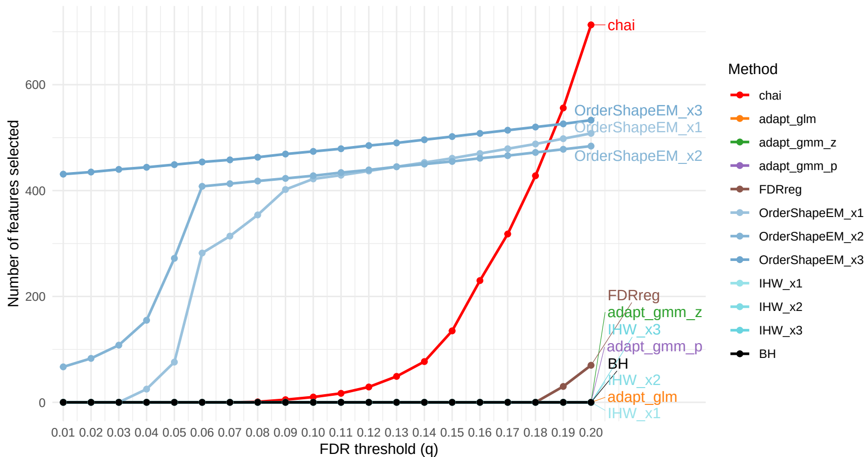
Feature Selection vs FDR (combined, unweighted, target=OTU, sideCov=Family)
