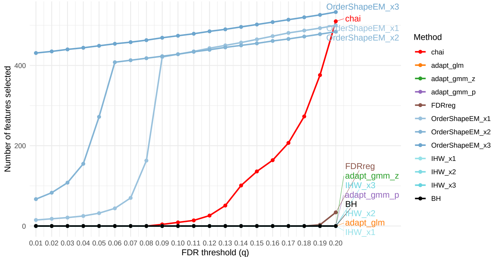
Feature Selection vs FDR (combined, unweighted, target=OTU, sideCov=Genus)
