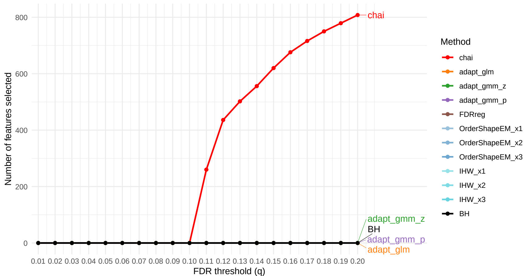
Feature Selection vs FDR (combined, unweighted, target=OTU, sideCov=Species)
