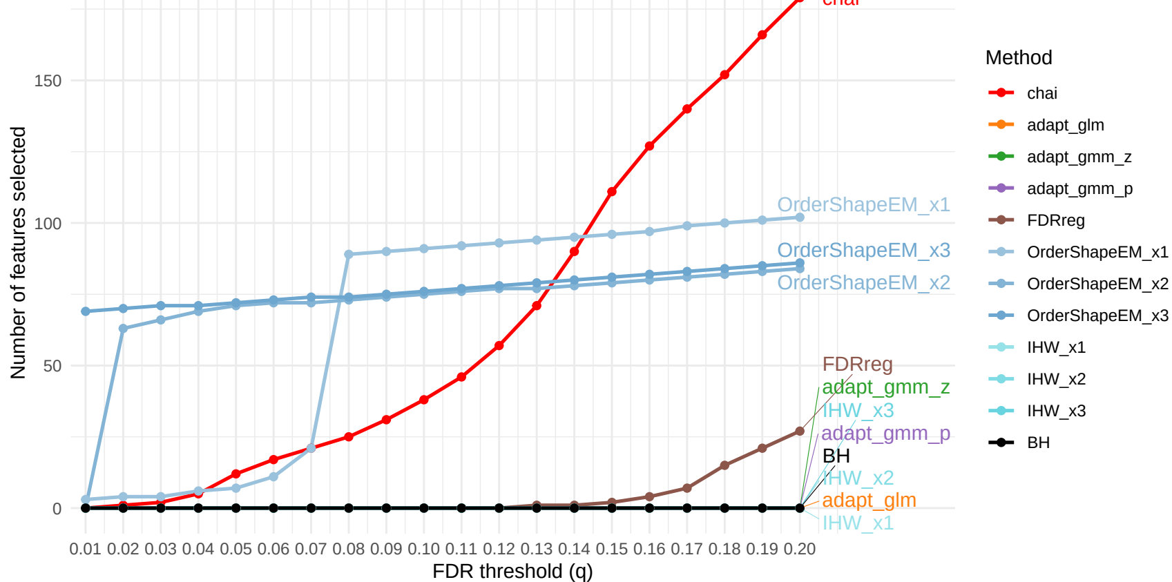
Feature Selection vs FDR (combined, unweighted, target=Species, sideCov=Genus)
