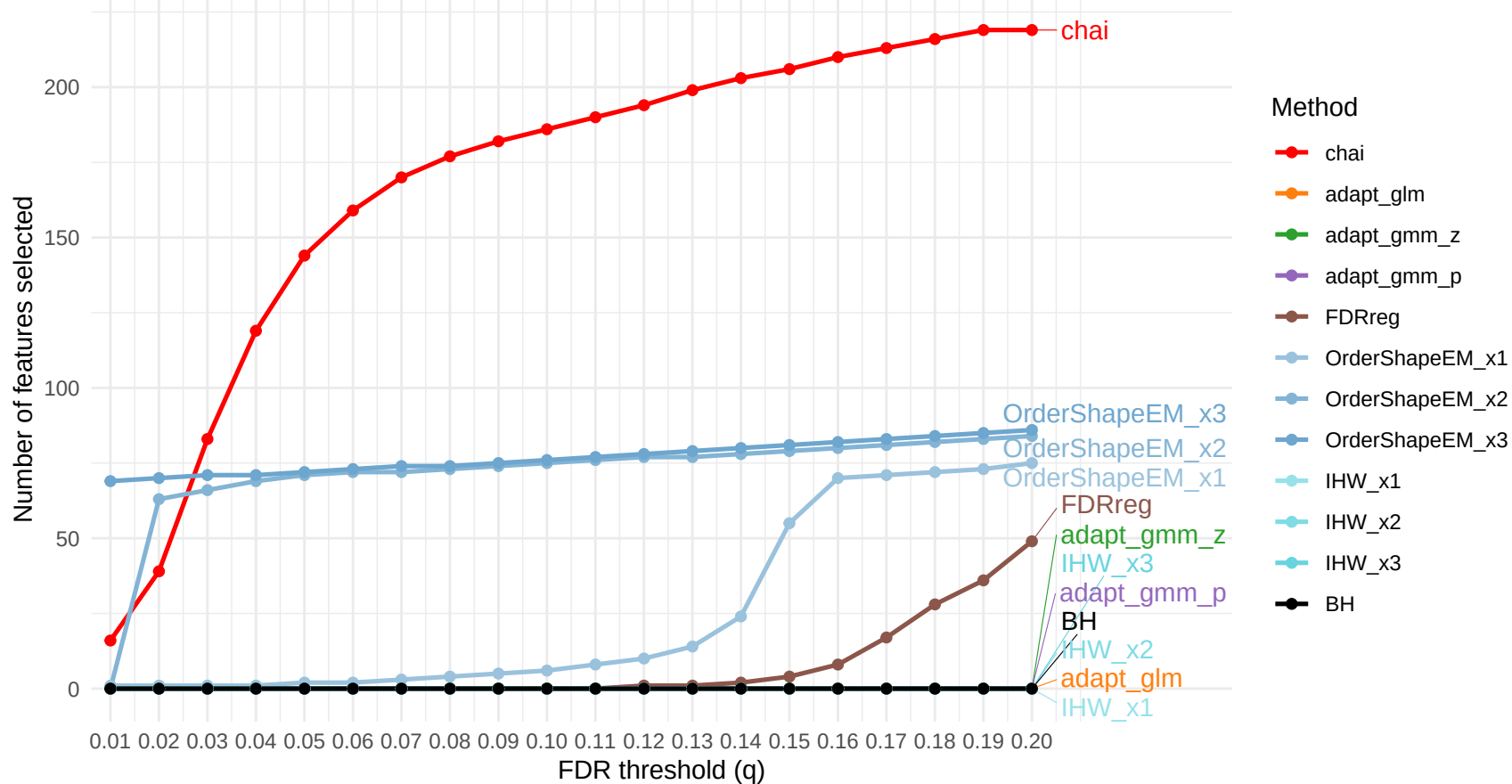
Feature Selection vs FDR (combined, unweighted, target=Species, sideCov=Order)
