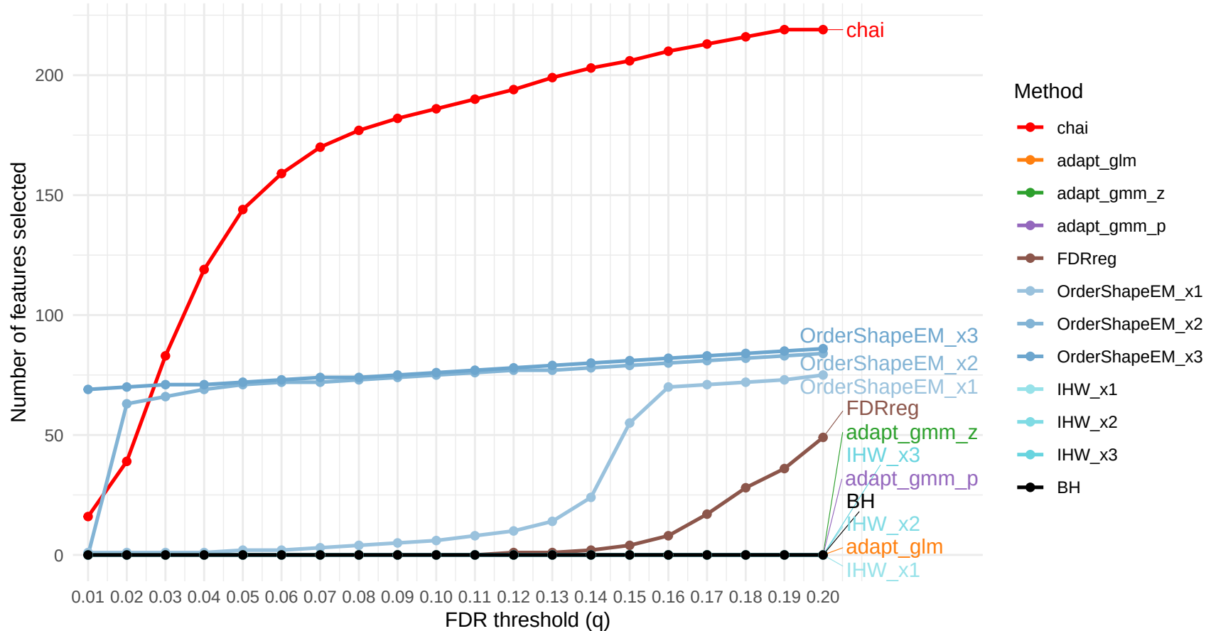
Feature Selection vs FDR (combined, unweighted, target=Species, sideCov=Phylum)
