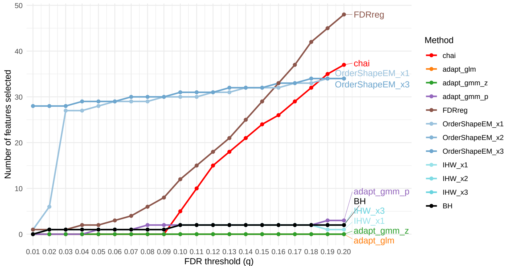
Feature Selection vs FDR (combined, weighted, target=Family, sideCov=Order)
