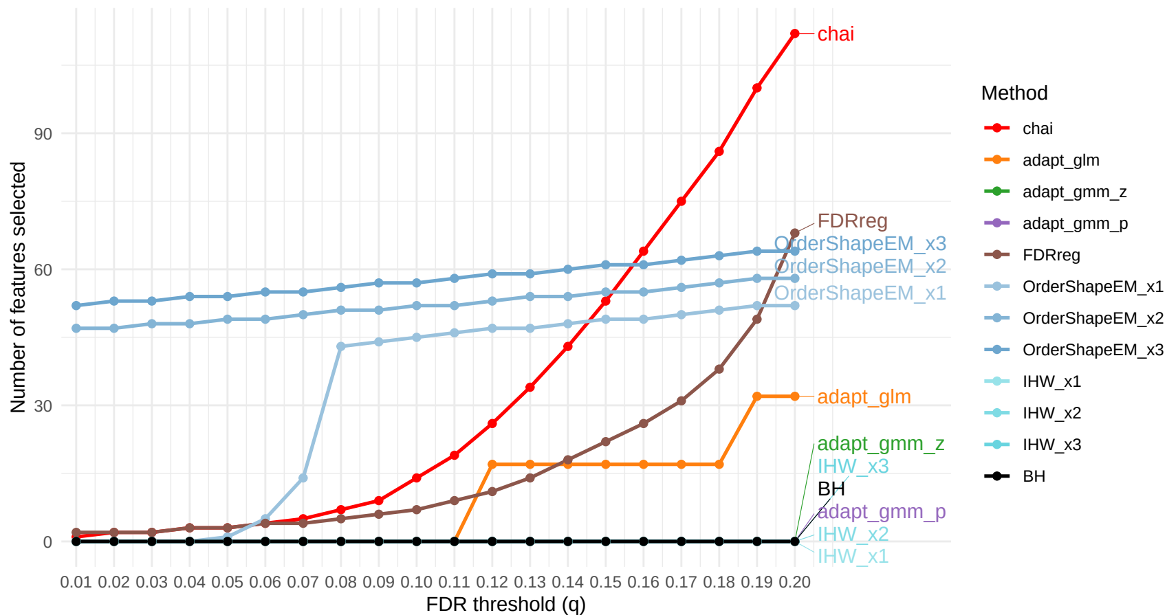
Feature Selection vs FDR (combined, weighted, target=Genus, sideCov=Class)
