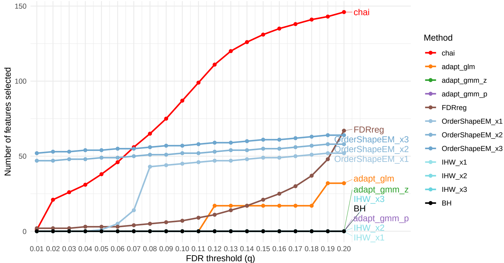
Feature Selection vs FDR (combined, weighted, target=Genus, sideCov=Family)
