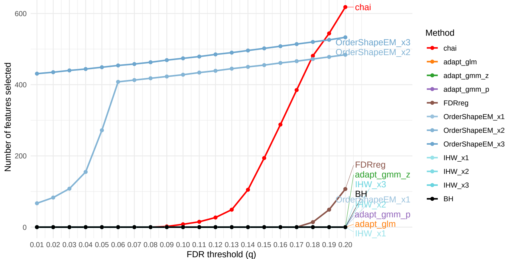
Feature Selection vs FDR (combined, weighted, target=OTU, sideCov=Phylum)
