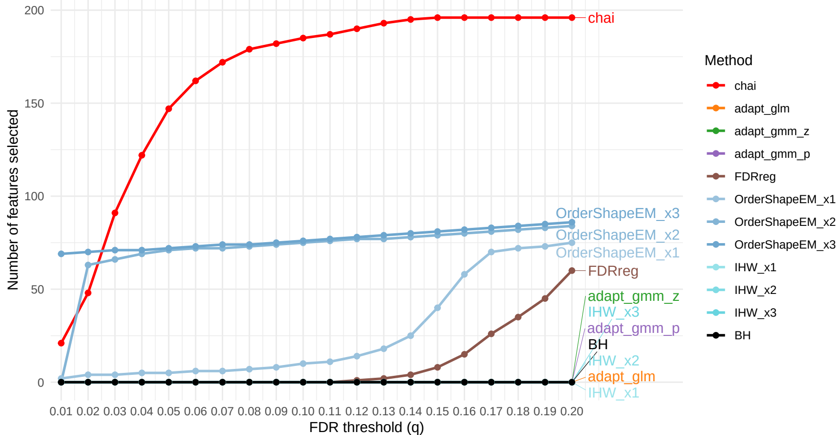
Feature Selection vs FDR (combined, weighted, target=Species, sideCov=Order)
