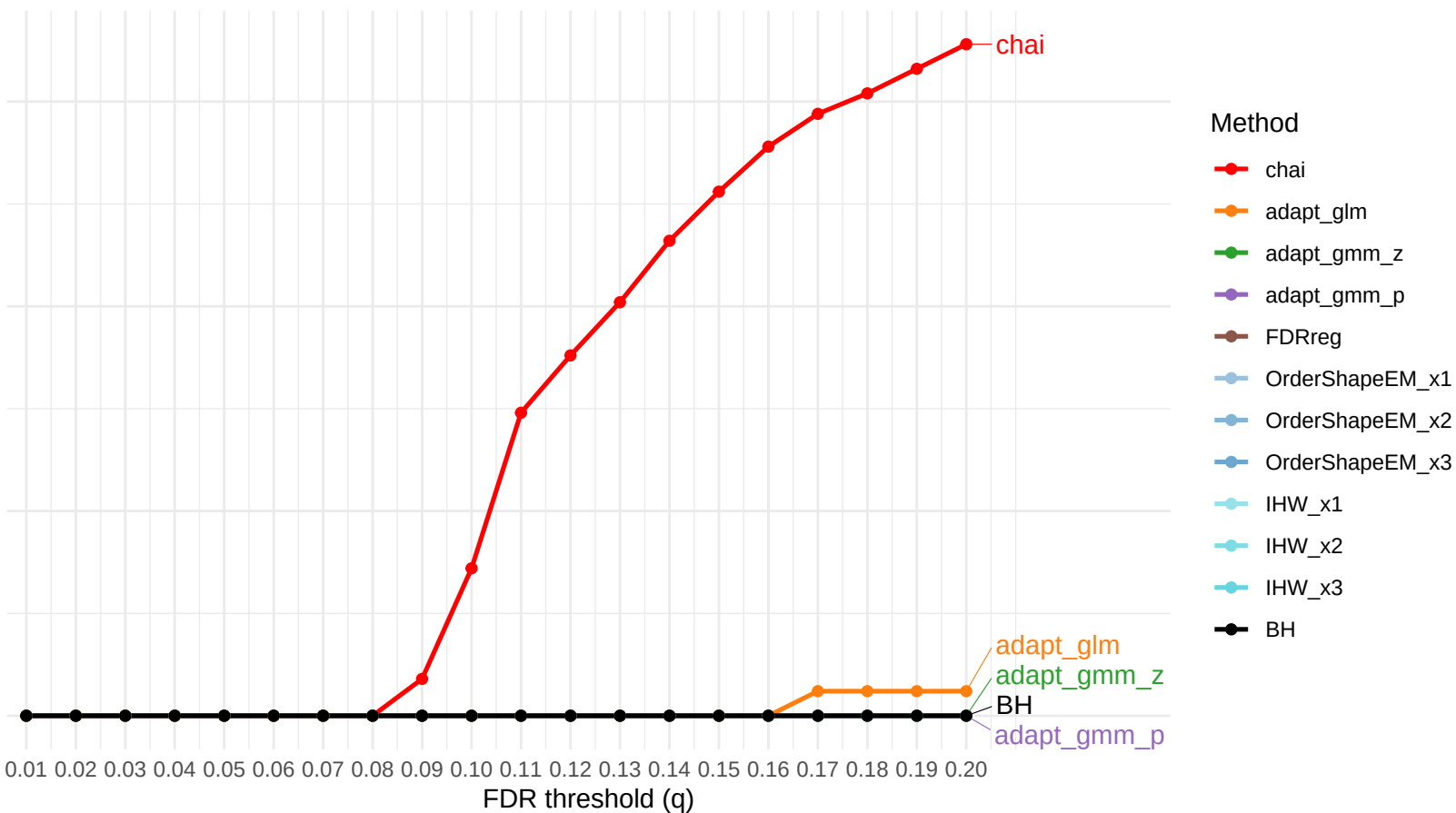
Feature Selection vs FDR (combined, weighted, target=Species, sideCov=Species)
