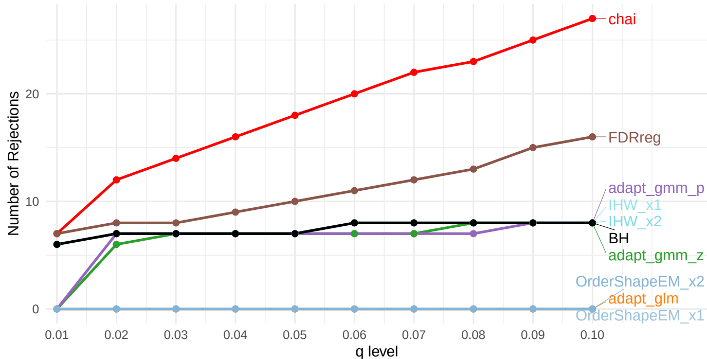
Number of Discoveries vs q, on DESeq2 statistics
