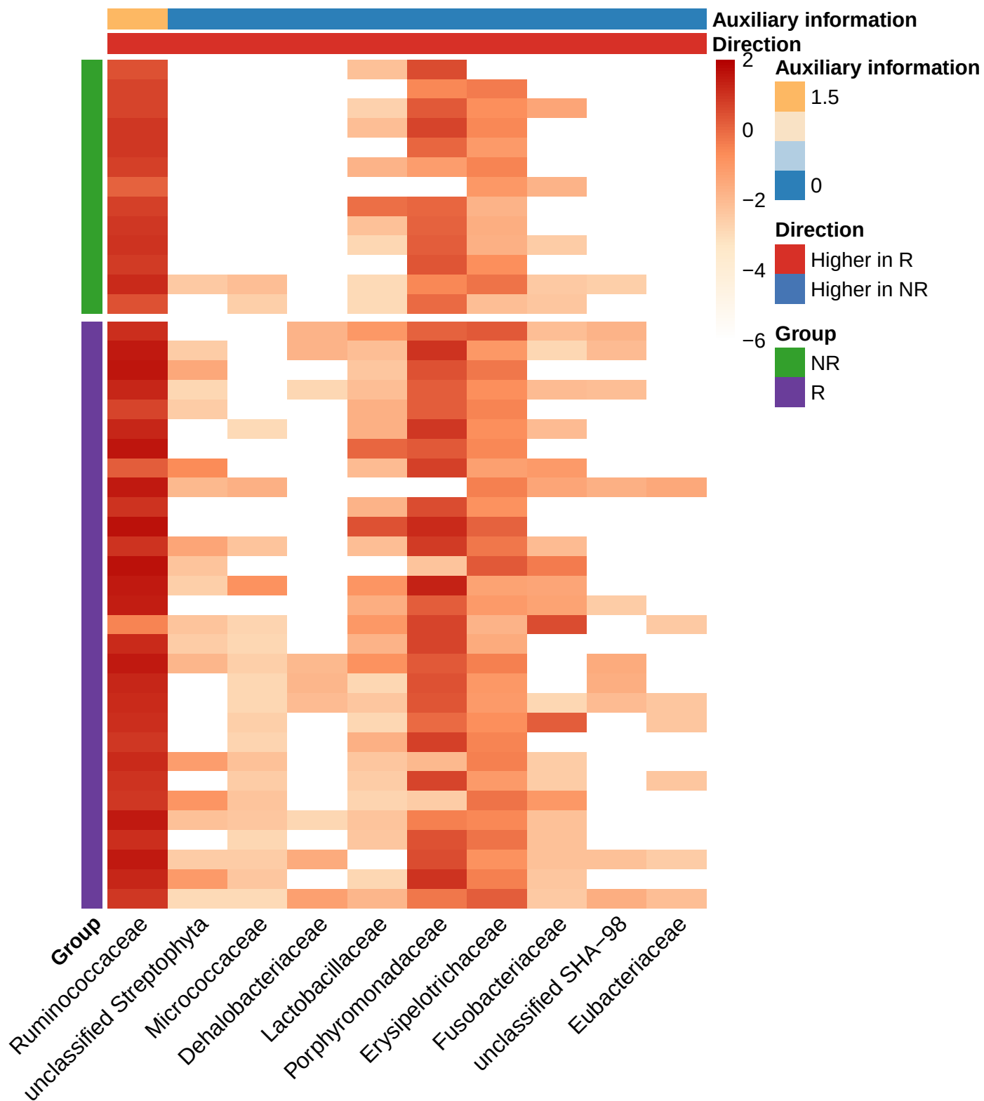
Top 10 features by |z|
