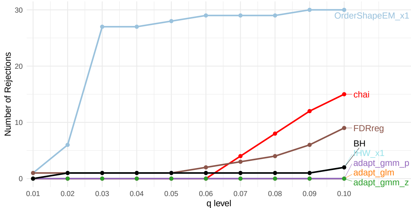
Number of Discoveries vs q , on Wilcoxon z -statistics
