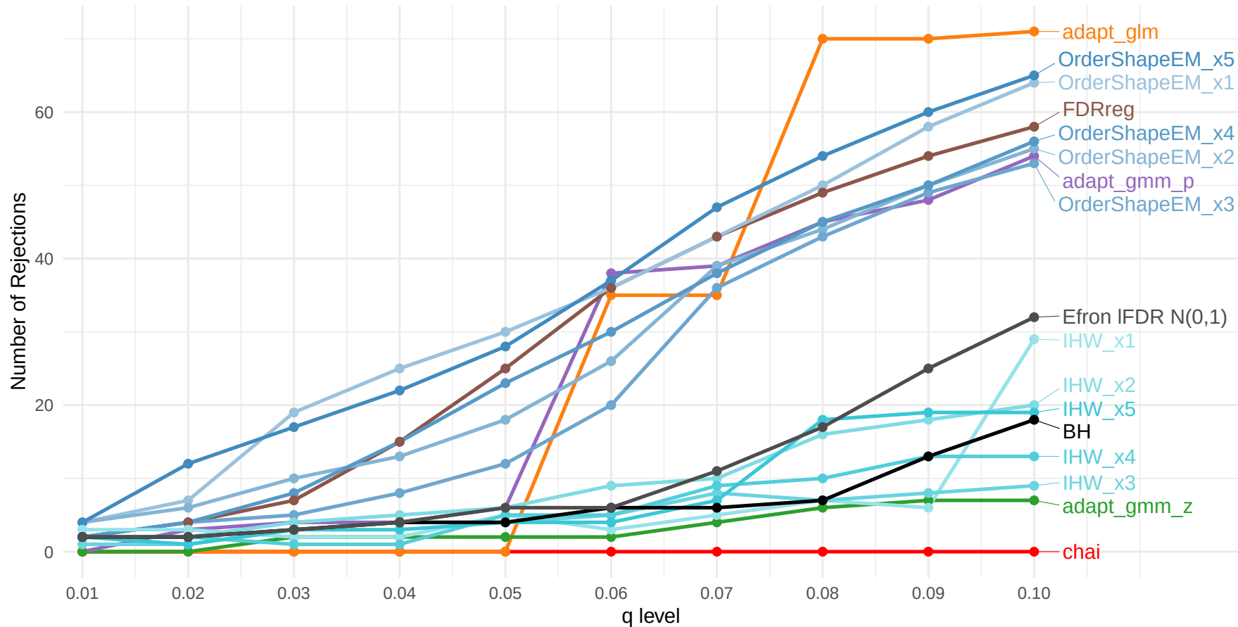
Number of Discoveries vs q, with Autoencoder
