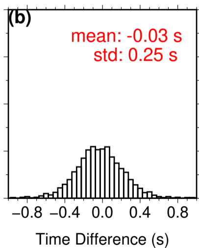
PhaseNet-TF (Iteration #2)
