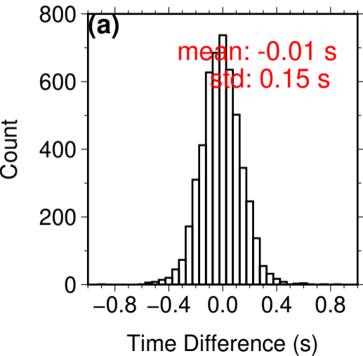
PhaseNet-TF (Iteration #1)
