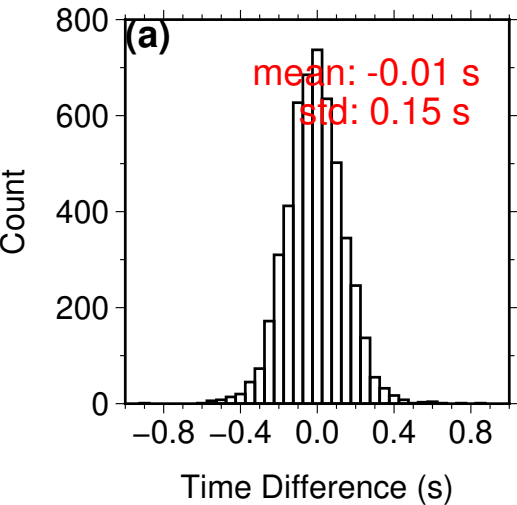
PhaseNet-TF (Iteration #1)
