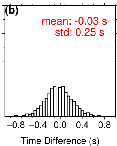
PhaseNet-TF (Iteration #2)
