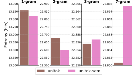
Figure 12: Semantic supervision does not consistently reduce empirical image-token n -gram entropy. The empirical entropy of the tokens is calculated on tokenized images of the LAION-Aesthetics validation set.
