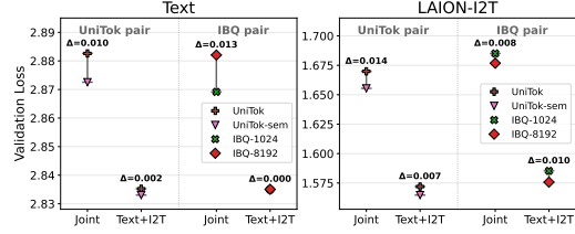
Figure 10: Changing the image token space can reduce interference between image-token and text-token modeling in joint training. In the joint setting, UniTok-sem and IBQ-1024 attain lower text loss than UniTok and IBQ-8192, respectively. When the image-generation objective is ablated (Text+I2T training), the text losses within each pair become similar (left), indicating that the interference stems from image-token modeling; the I2T gap, however, persists (right).
