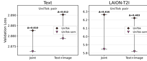
Figure 22: In the joint modeling setting, UniTok-sem has lower text loss than UniTok. In Text+T2I training ablating the I2T task, the gap is not reduced, suggesting that the interference does not come from the I2T task. As a side finding, the I2T task complements text modeling in joint training for both tokenizers.
