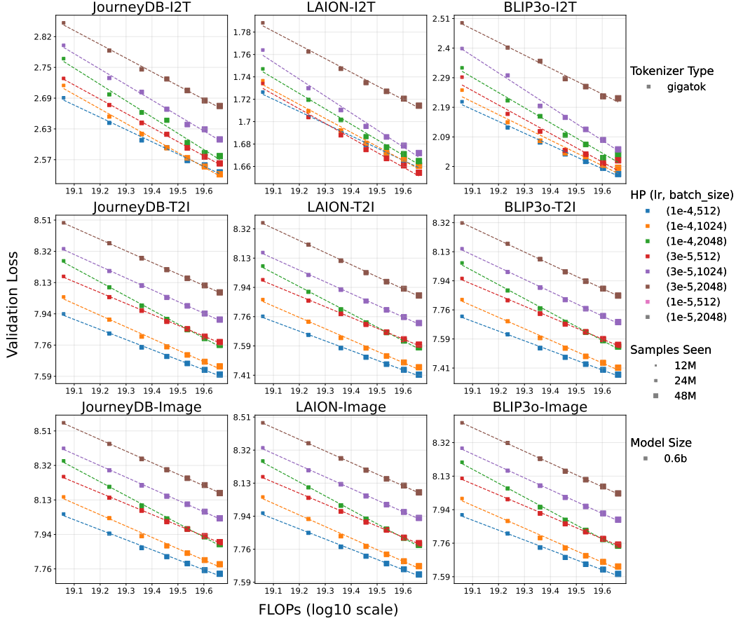
Figure 18: Loss scales with data similarly for image-text data from different sources.
