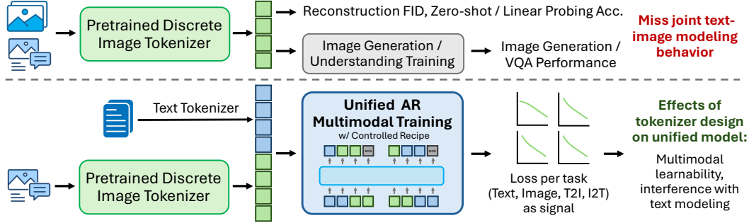
Figure 1: Studying image tokenizers as visual languages in unified multimodal models. Prior tokenizer studies focus on downstream-agnostic metrics (reconstruction/probing) or single-axis generation-/understanding-only pipelines, which miss joint text–image modeling behavior. We study tokenizers in the context of unified AR multimodal training, using task-specific losses as a signal to reveal how the tokenizer shapes downstream joint modeling.
