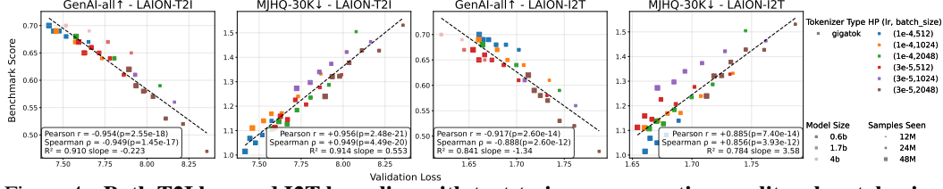
Figure 4: Both T2I loss and I2T loss align with text-to-image generation quality when tokenizer type is controlled. The lines are linear fits to all dots.
