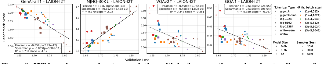
Figure 9: I2T loss shows moderate correlation with both generation and understanding performance after SFT across tokenizers. We use the checkpoints after annealing for loss evaluation.
