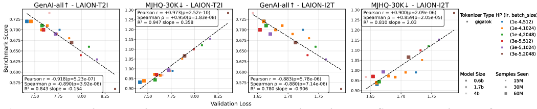
Figure 8: Both I2T and T2I loss show strong correlation with post-SFT generation performance when tokenizer type is controlled. We use the checkpoints after annealing for loss evaluation.
