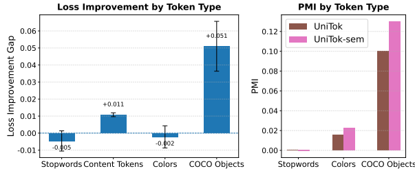
Figure 11: Semantic supervision strengthens object-level image-token-word alignment (“better visual words”). UniTok-sem yields larger I2T loss improvements on COCO object words than on stopwords, colors, or general content tokens (left), and higher PMI between image tokens and object words (right).
