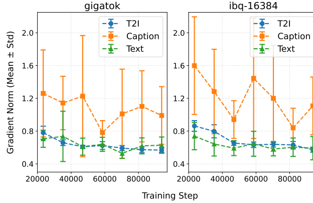
Figure 17: Gradient norms over all parameters by modality across training steps of 0.6B model with GigaTok and IBQ-16384 ( lr=3e-5 , bs=512 ). For both runs, the T2I gradient slowly saturates at the end.
