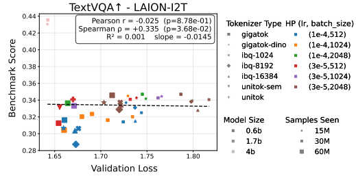
Figure 21: I2T loss has a noisy and inconsistent correlation with TextVQA performance.
