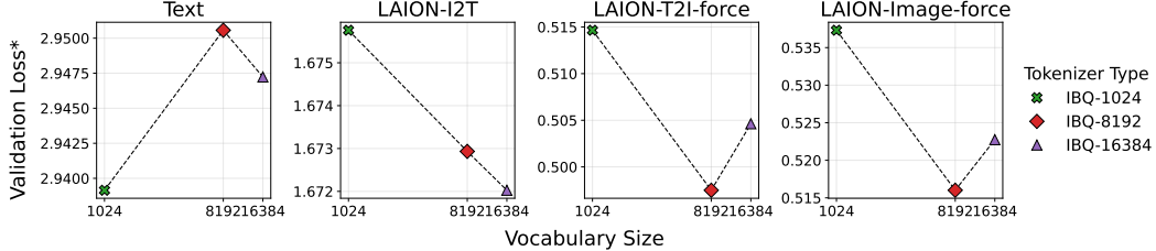
Figure 13: Vocabulary size changes task-specific validation losses with no simple monotonic trend. Among the three IBQ variants, IBQ-16384 achieves the best I2T loss, but IBQ-8192 attains the lowest T2I and image losses after normalization ( \text{lr}=1\text{e-}4 , batch size=512).
