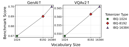
Figure 14: The largest vocabulary brings the best downstream performance among the three IBQ variants ( \text{lr}=1\text{e-}4 , batch size=512).
