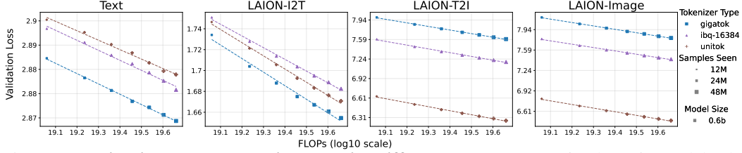
Figure 2: Validation losses scale with data size differently across tasks for the 0.6B model. The y-axis is in log scale. The lines are linear fits to the dots per tokenizer.
