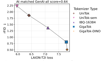
Figure 7: The T2I loss–performance relation shift is related to differences in reconstruction fidelity. The rFID is negatively correlated with T2I loss when the GenAI benchmark score is controlled.
