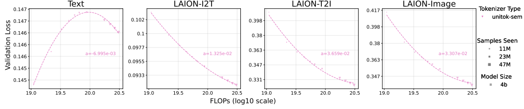
Figure 16: Quadratic fitting of UniTok-sem 4B training, including data points from earlier stage of continual training.
