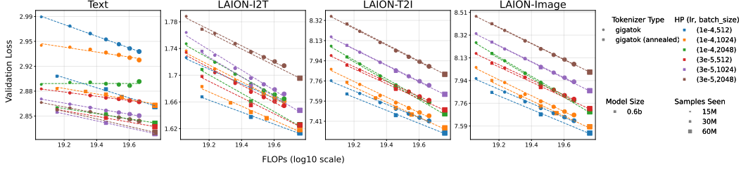
Figure 20: Loss scales with data for annealed and non-annealed checkpoints.
