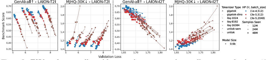
Figure 5: T2I loss does not align with text-to-image generation quality across tokenizers (the first two plots), while I2T loss aligns with generation quality (the last two plots). The lines are linear fits to the dots per tokenizer and per hyperparameter.
