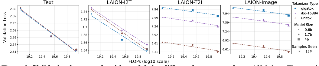
Figure 3: Validation losses scale with model size differently across tasks on 12M data. The y-axis is in log scale. The lines are linear fits to the dots per tokenizer.
