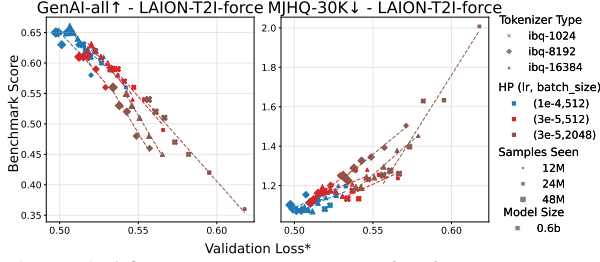
Figure 6: After vocabulary normalization, a more consistent T2I loss–performance relation exists across IBQ tokenizers. The lines are linear fits to the dots per hyperparameter. Quantitative results are in Table 10.
