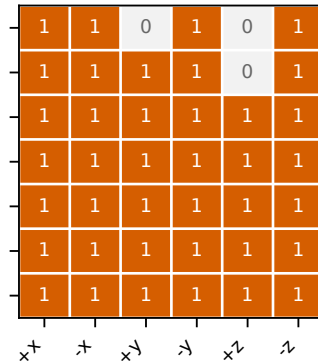
ReaxFF rerun
