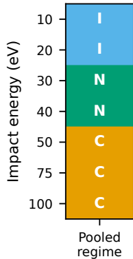
A DFT/MM
