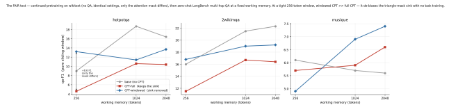
Figure 8: LongBench multi-hop QA (Qwen2.5-0.5B, continued-pretraining, no task supervision). At a tight window the windowed model uses a bounded working memory better than a full-attention control; the gap shrinks as the window grows.
