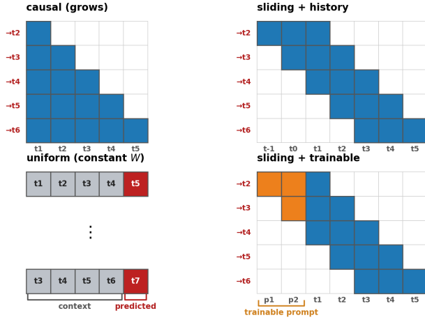
Figure 2: Four continued-pretraining regimes (blue = the attention mask in the matrix panels; grey = a context token and crimson the predicted token in the uniform sequence panel). Top, attention masks (rows = a predicting step, columns = attended positions; both predict every token): the standard causal mask, where context grows with position; and a sliding window of constant width W whose cold start is filled with real prior text (blue, the same as content — history is just earlier context). Bottom: the uniform window is not an attention mask but fixed-length training — a stack of fixed-length sequences (two windows shown with aligned boxes
