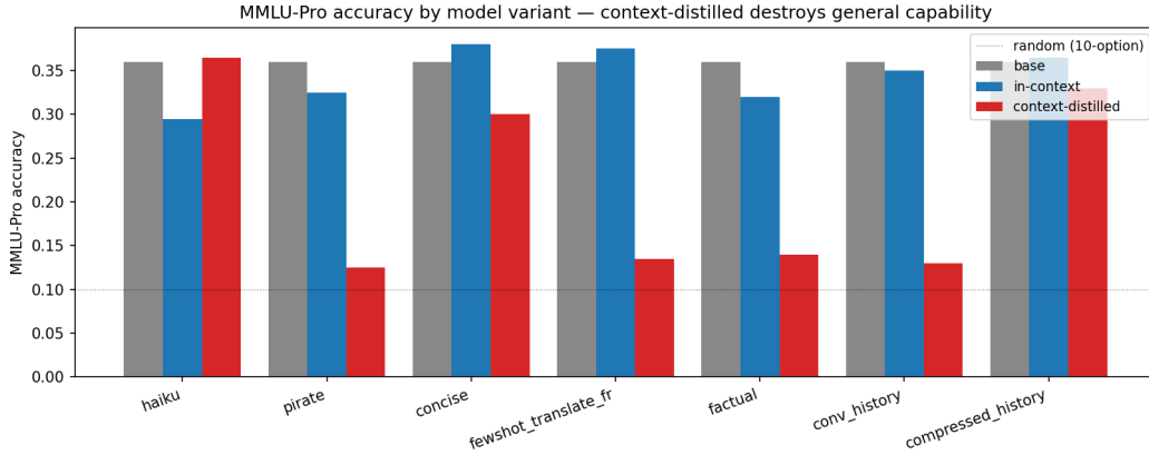
Figure 7: MMLU-Pro accuracy by model variant. Gray = base, blue = in-context, red = context-distilled. Dotted line = random-guess for 10-option MCQ. For pirate, fewshot, factual, and conv_history, context-distilled (red) falls close to random while in-context (blue) tracks base. Only haiku and compressed_history avoid the catastrophic drop.
