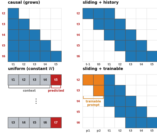
Figure 2: Four continued-pretraining regimes (blue = the attention mask in the matrix panels; grey = a context token and crimson the predicted token in the uniform sequence panel). Top, attention masks (rows = a predicting step, columns = attended positions; both predict every token): the standard causal mask, where context grows with position; and a sliding window of constant width W whose cold start is filled with real prior text (blue, the same as content — history is just earlier context). Bottom: the uniform window is not an attention mask but fixed-length training — a stack of fixed-length sequences (two windows shown with aligned boxes and shifted token indices, \vdots for the rest), each predicting only its last token (crimson) from its preceding context, so it also runs on a recurrence; and a sliding window with trainable tokens , whose cold start is filled by a trainable startup prompt (orange) that slides out as content accumulates. Older real context must be carried by the weights.
