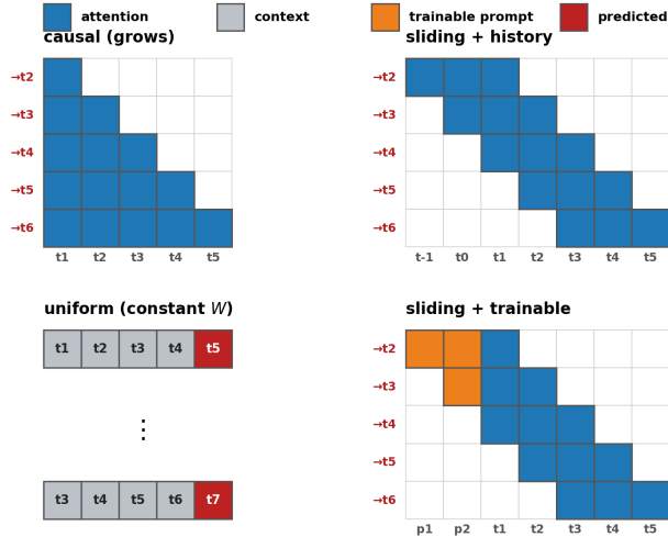
Figure 2: Four continued-pretraining regimes (blue = the attention mask in the matrix panels; grey = a context token and crimson the predicted token in the uniform sequence panel). Top, attention masks (rows = a predicting step, columns = attended positions; both predict every token): the standard causal mask, where context grows with position; and a sliding window of constant width W whose cold start is filled with real prior text (blue, the same as content — history is just earlier context). Bottom: the uniform window is not an attention mask but fixed-length training — a stack of fixed-length sequences (two windows shown with aligned boxes and shifted token indices, \vdots for the rest), each predicting only its last token (crimson) from its preceding context, so it also runs on a recurrence; and a sliding window with trainable tokens , whose cold start is filled by a trainable startup prompt (orange) that slides out as content accumulates. Older real context must be carried by the weights.
