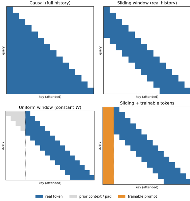
Figure 2: Four continued-pretraining regimes, shown as attention masks (each query row attends its shaded key columns). Top : the standard causal mask (full, growing history) and a sliding window of width W over real recent history. Bottom, our constant-memory variants : a uniform window , where every token is conditioned on exactly W tokens via fixed-length training, so it also runs on a recurrence (early tokens padded, grey); and a sliding window with trainable tokens , where an always-on or cold-start trainable prefix (orange) replaces the sink. Older real context must be carried by the weights.
