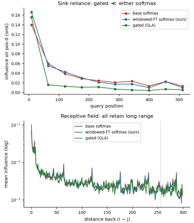
Figure 7: Cross-architecture attention pattern (fla 1.3B, gradient influence at full attention). Left: the gated model places far less influence on the position-0 sink than either softmax model; base and our windowed-FT softmax coincide — windowed training does not intrinsically remove the sink, the deployment window does. Right: all three retain long-range influence (overlapping decay); the sink, not the receptive field, is the distinguishing feature.
