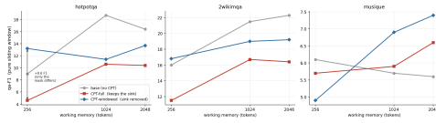
Figure 8: LongBench multi-hop QA (Qwen2.5-0.5B, continued-pretraining, no task supervision). At a tight window the windowed model uses a bounded working memory better than a full-attention control; the gap shrinks as the window grows.
