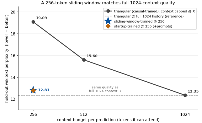
Figure 4: Held-out perplexity vs. deployed working-memory window (Qwen2.5-0.5B). The base model collapses as the window shrinks; the windowed-finetuned model is nearly flat and matches full-context quality at a small window.
